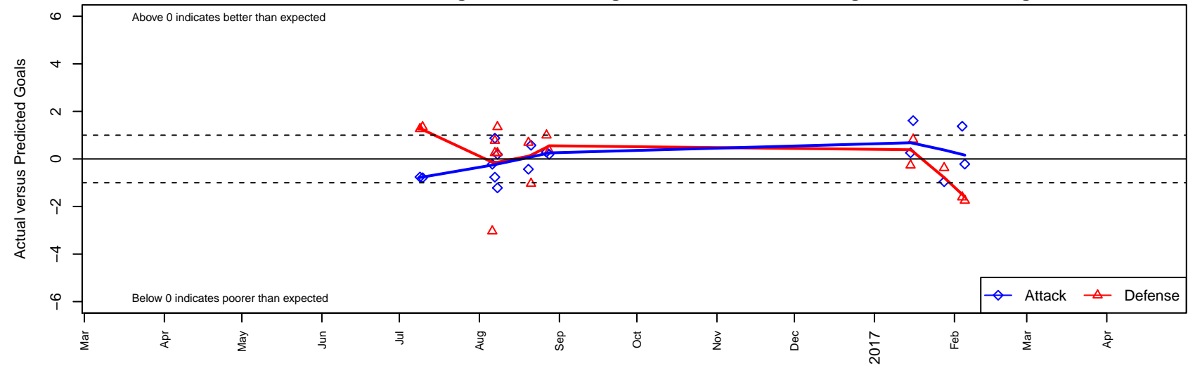
LA Galaxy SD Elite G03 Dots are actual minus expected GF (blue circles) and GA (red triangles). Blue line is smoothed change in attack strength. Red is smoothed change in defense strength.
